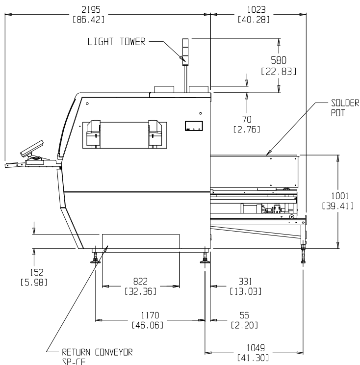
Figure 3: Load and Unload End Views
